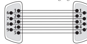
Straight-through configuration cable with handshaking signals
