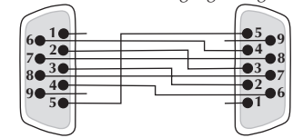
Null-modem configuration cable with handshaking signaling
