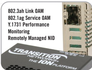
10/100/1000BASE-TX to 1000BASE-X OAM/IP-Based Remotely Managed NID
